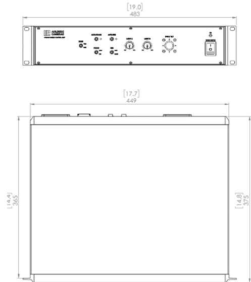
Figure 2 - CCU100 dimensions
